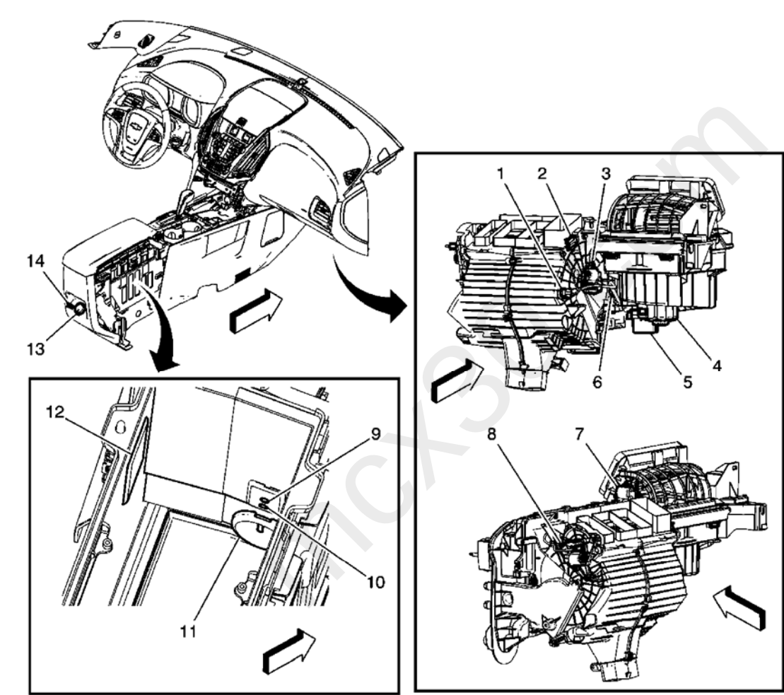
Fig. 3: Identifying Right Side of Instrument Panel - Center Console and HVAC System Courtesy of GENERAL MOTORS CORP.
